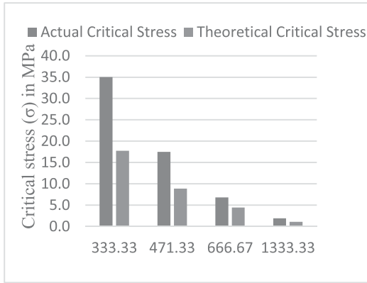
Fig. 4: \frac{L_e}{r} Vs Critical Stress in MPa
