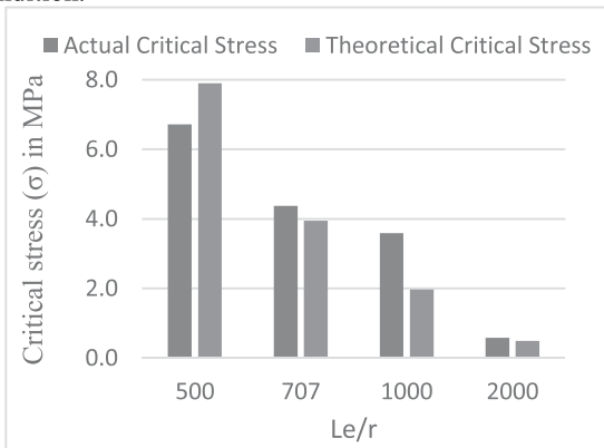
Fig. 18: \frac{L_e}{r} Vs Critical Stress in MPa.
