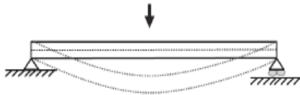
Fig. 1: Bending deformation[14]
