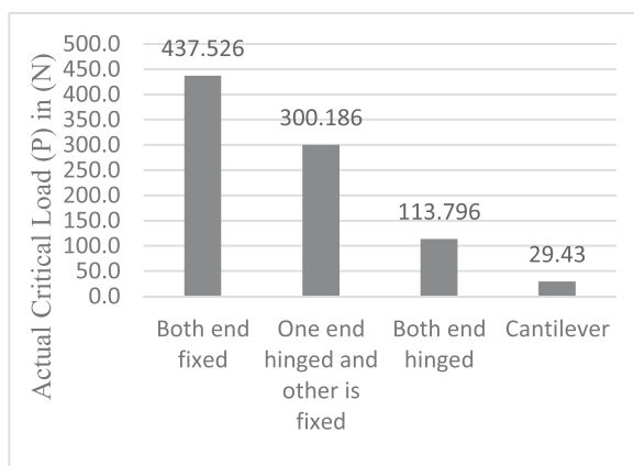
Fig. 15: Support Conditions Vs Critical Load (P) in (N)
