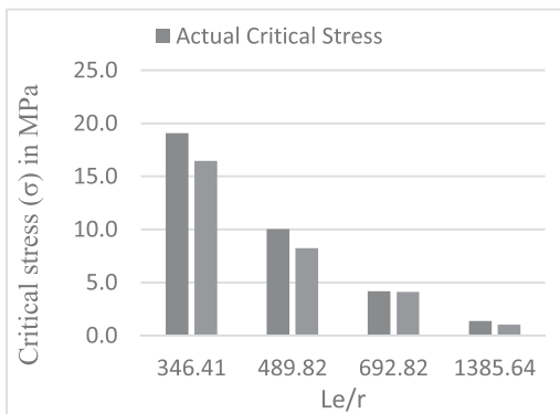
Fig. 26: \frac{Le}{r} Vs Critical Stress in MPa.
